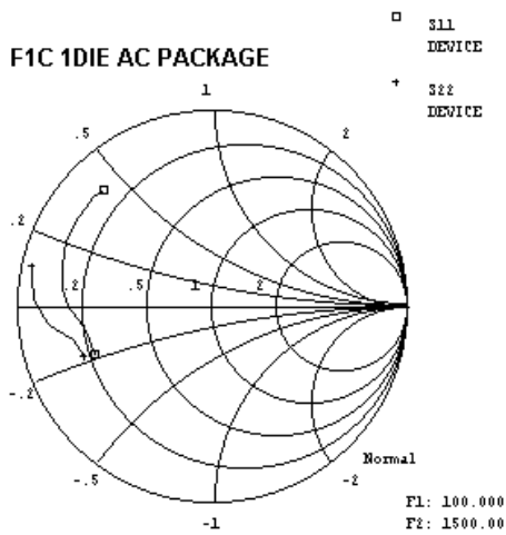
S11 AND S22 SMITH CHART
