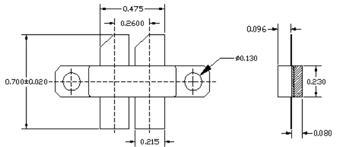
PACKAGE DIMENSIONS IN INCHES
