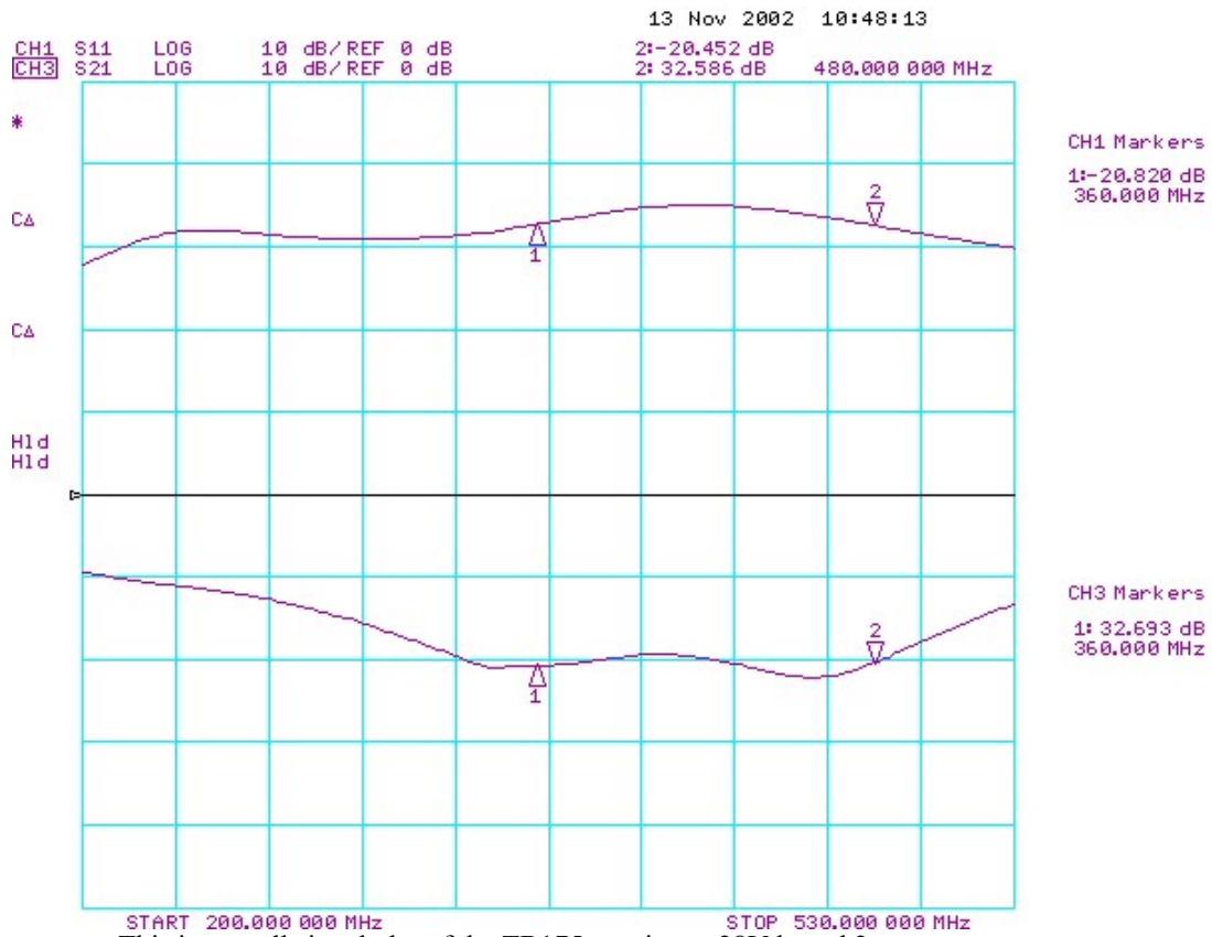
This is a small signal plot of the TB175 running at 28Vdc and 2 amps.
