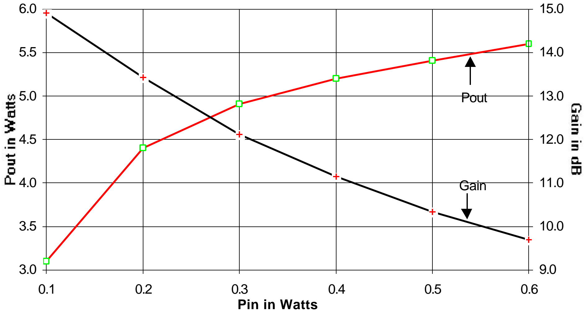
TB-211 Pin vs Pout Freq=300MHz Vds=7.5 Vdc
