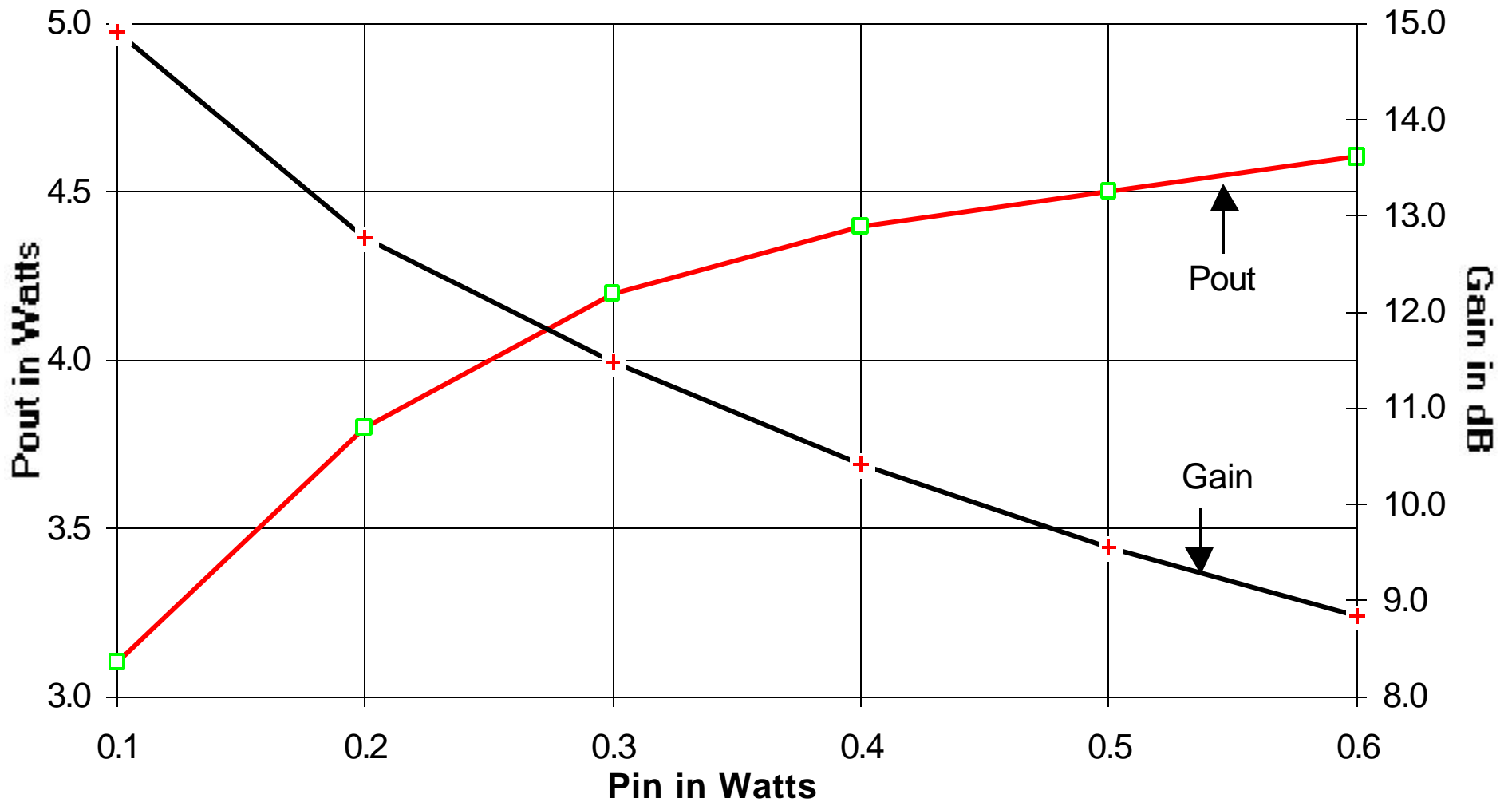
TB-211 Pin vs Pout Freq=400MHz Vds=7.5 Vdc
