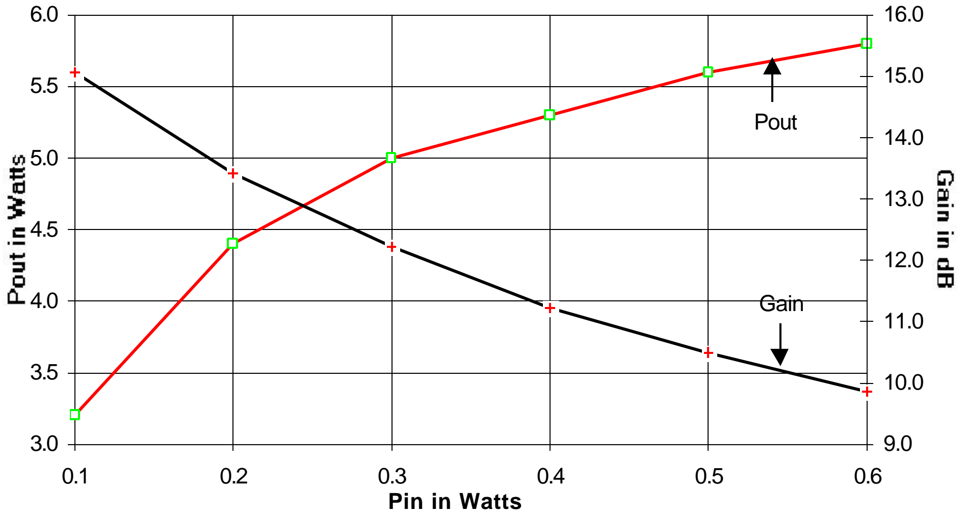
TB-211 Pin vs Pout Freq=350MHz Vds=7.5 Vdc
