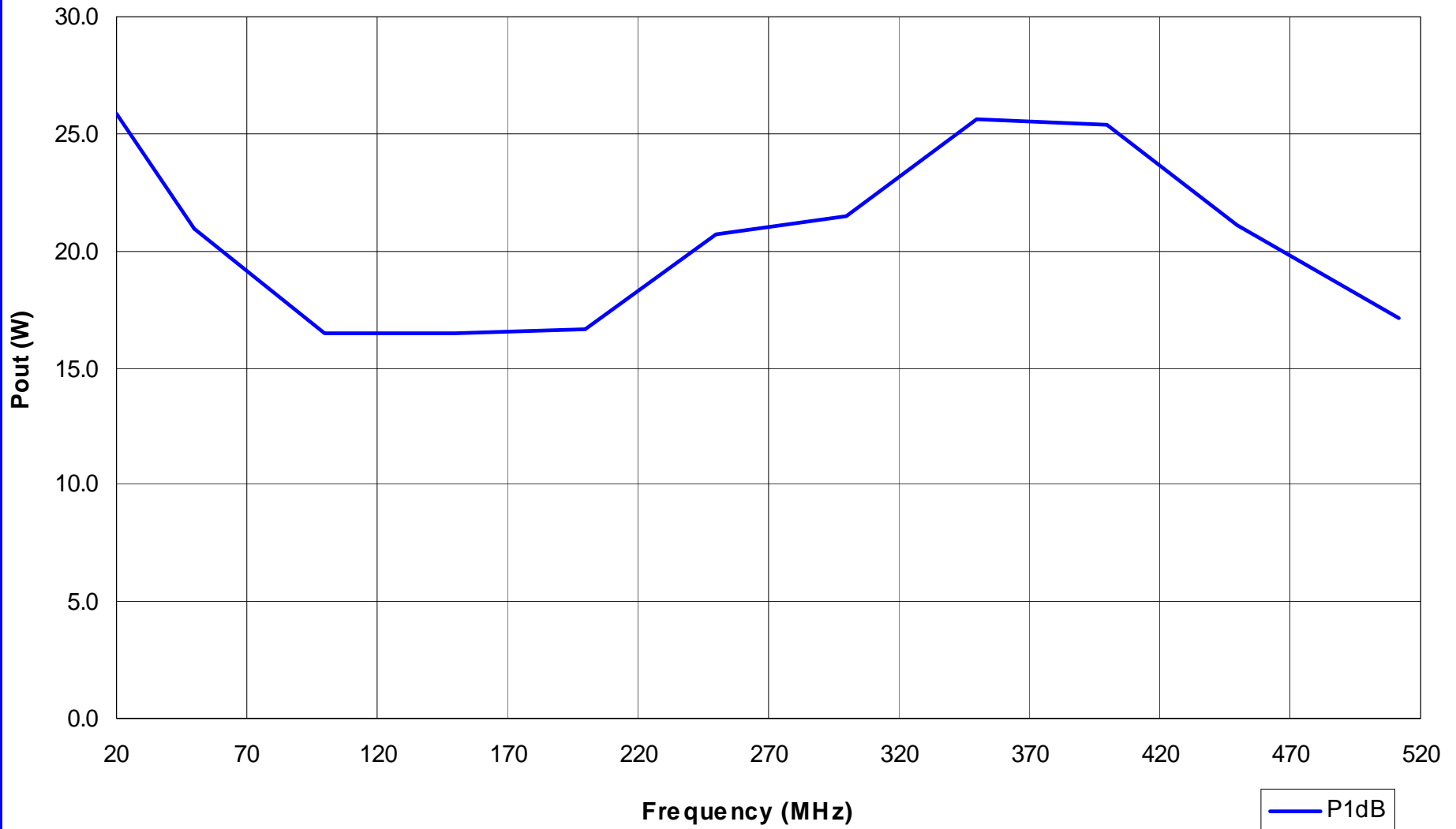
TB219#3 LQ801 P1dB vs Frequency: Vds=28Vdc, Idq=200mA
