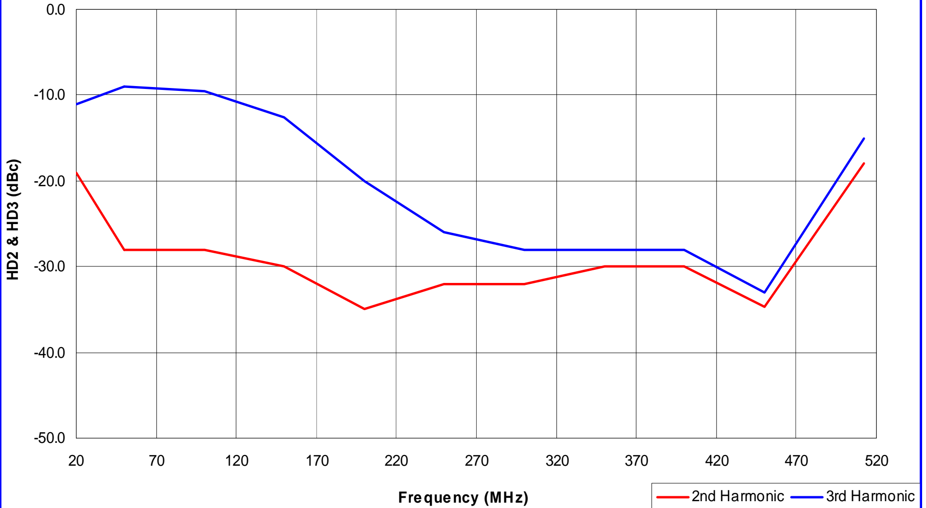
TB219#3 LQ801 Harmonics vs Frequency: Vds=28Vdc, Idq=200mA, Pout=20W
