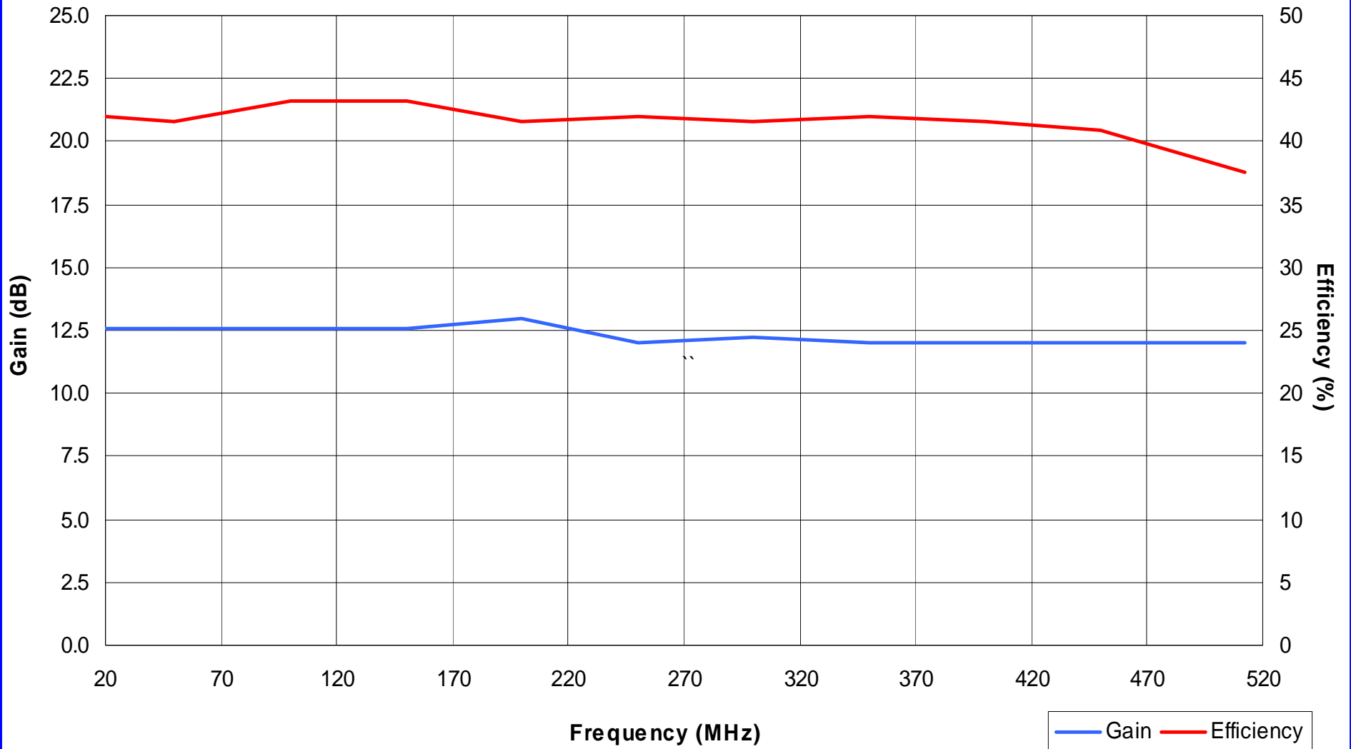
TB219#3 Gain/Efficiency vs Frequency: Vds=28Vdc, Idq=200mA, Pout=20W
