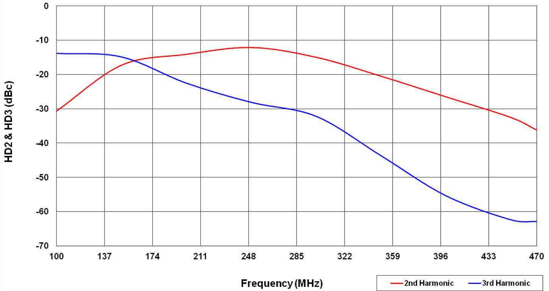
TB231 Harmonics vs Frequency: V_{ds} = 28V_{dc} , I_{dq} = 200mA , P_{out} = 10W
