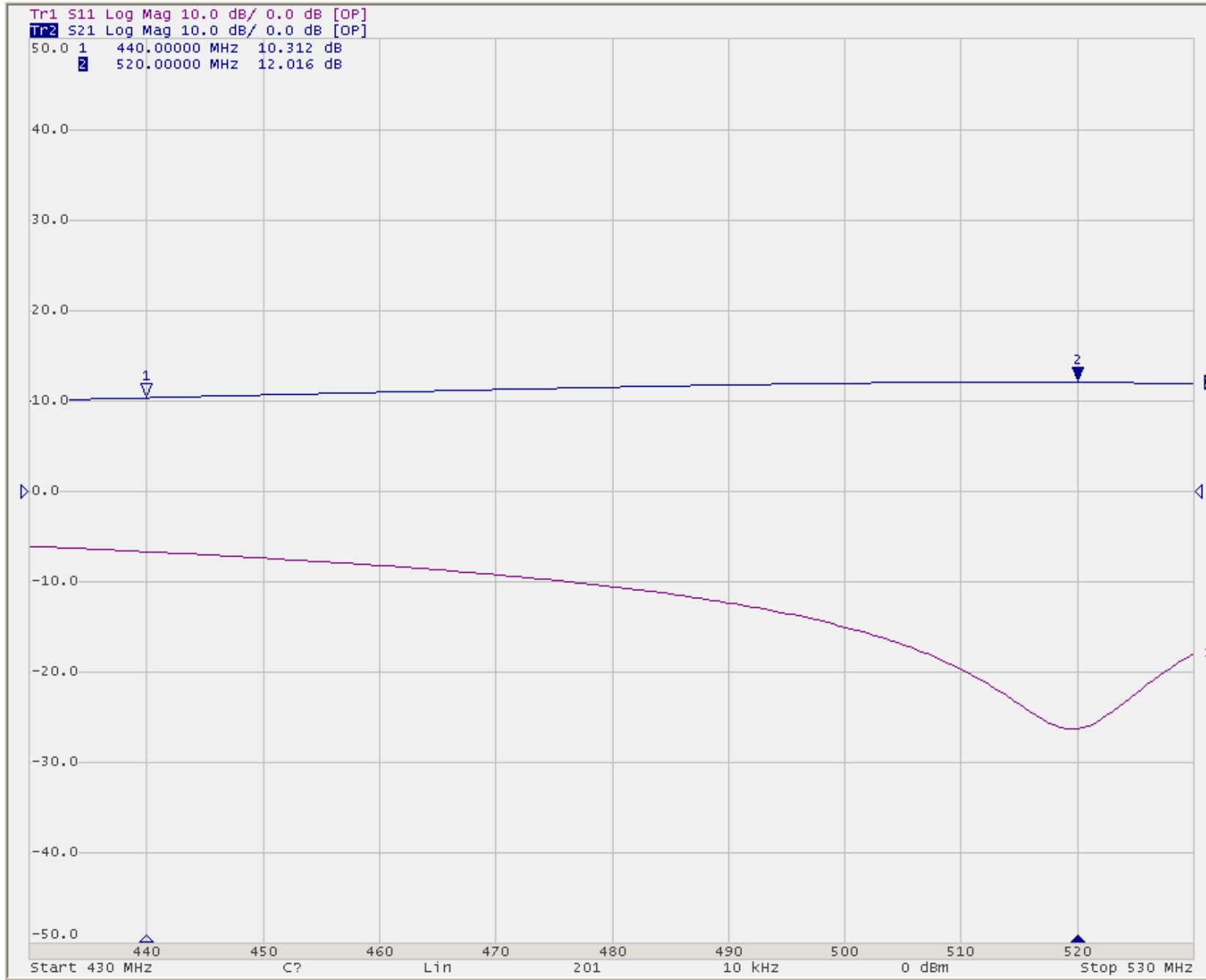
TB236: Vds=28Vdc, Idq=0.6A, Pin=0dBm
