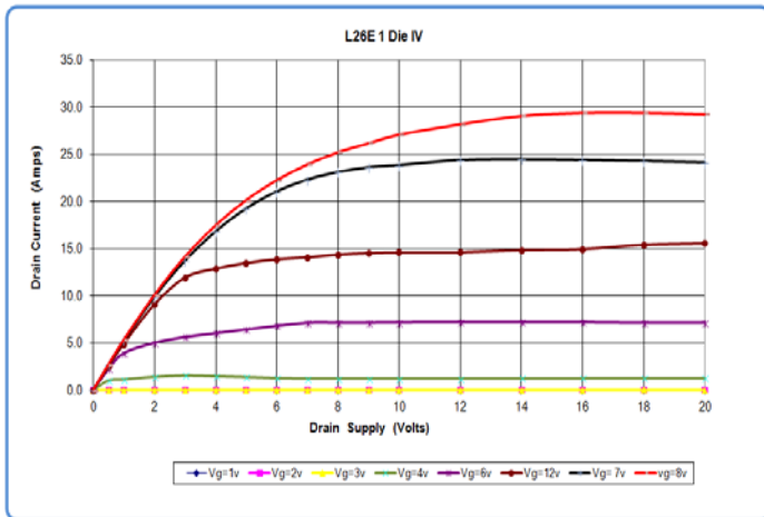
IV CURVE
