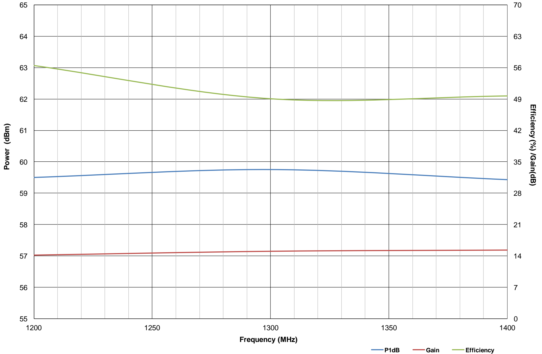
TB277C :LY2542LR P1dB /Gain/Efficiency vs. Frequency: Vds = 50VDC, Idq = 90mA, D.C. = 10%, Pulse Width = 180us
