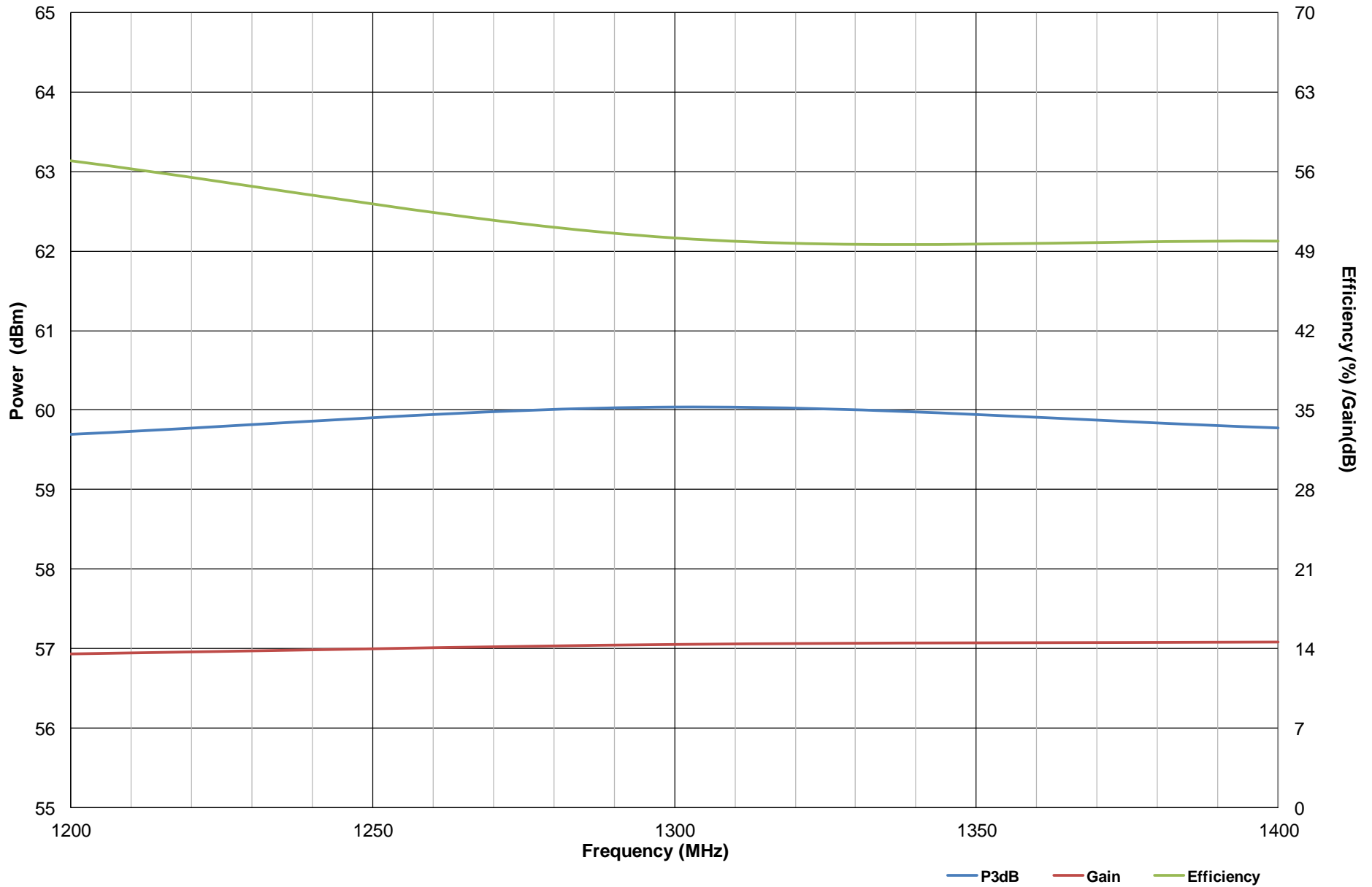
TB277C: LY2542LR P3dB /Gain/Efficiency vs. Frequency: Vds = 50Vdc, Idq = 90mA, , D.C. = 10%, Pulse Width = 180us
