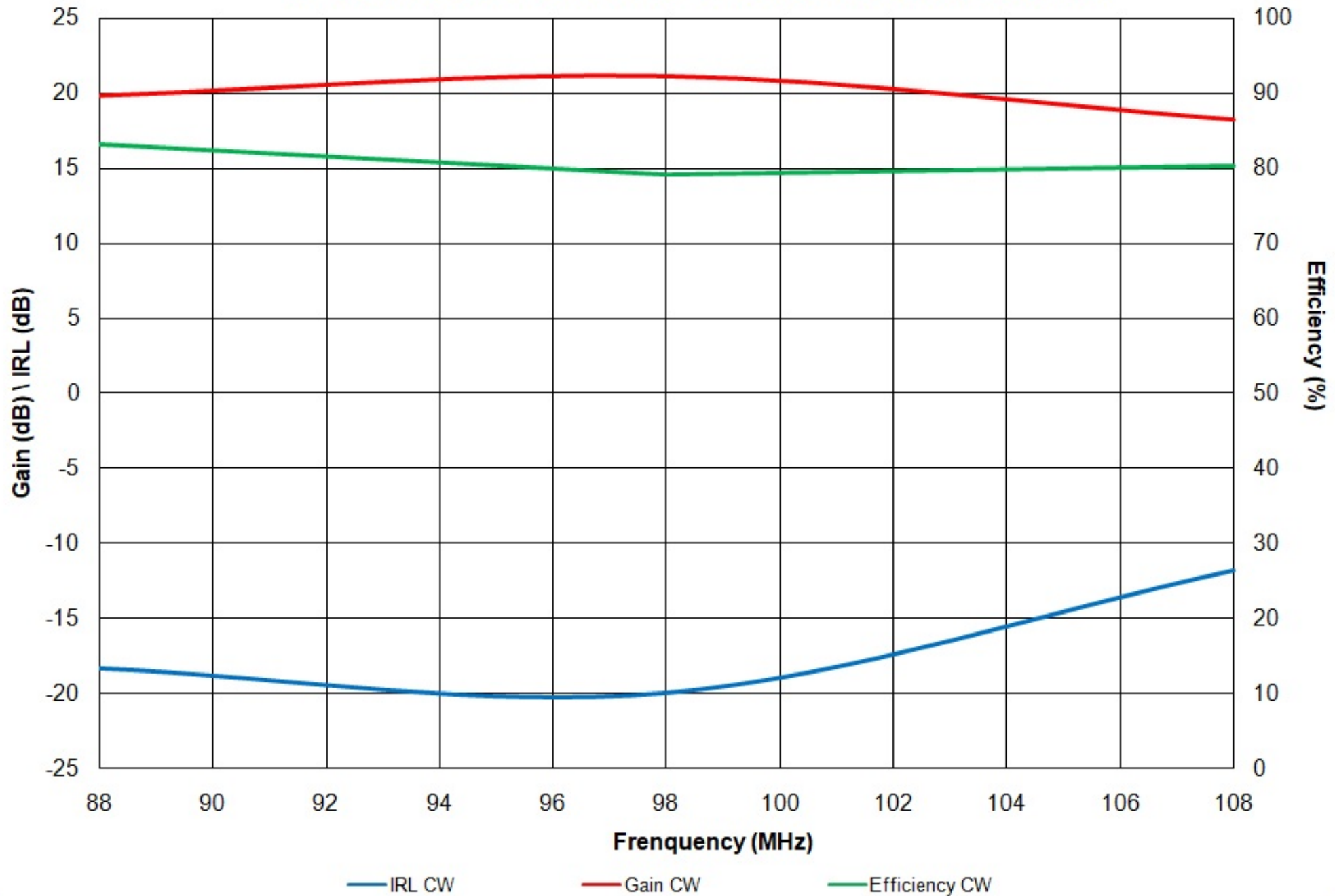
Gain/IRL/Efficiency vs Frequency : Vds = 50VDC, Idq = 200mA, Pout = 2000 Watts
